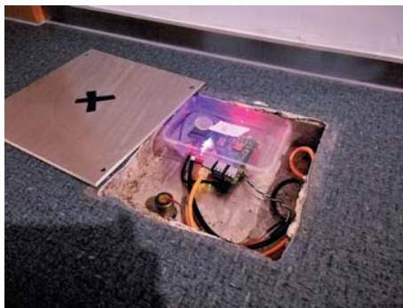
Figure 3: Deployed sensing unit example: For safety reason, sensing unit is installed underneath the floor, and covered with a steel plate. The geophone sensor is fixed on the floor to ensure a stable connection.
